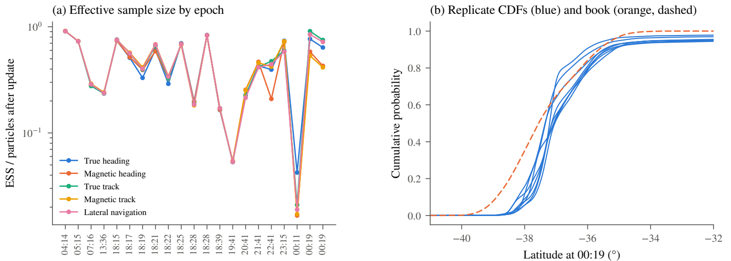
Figure 4. (a) Effective sample size after each measurement update, averaged over replicates, per autopilot-mode filter. The narrowest bottlenecks are the 18:39 C-channel BFO (the southward turn) and the 19:41 BTO arc. (b) Latitude CDFs of the 8 independent replicates; the largest difference between any two is 0.227 (Kolmogorov distance).
